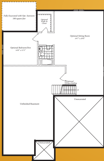
Optional Basement Upgrade: 915 Square Feet
