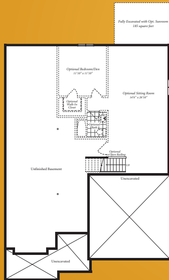
Optional Basement Upgrade Elevation A 762 Square Feet
